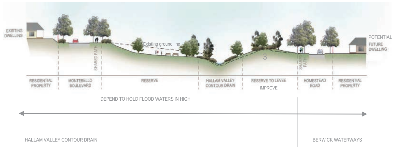
Cross section of ultimate levee bank works
